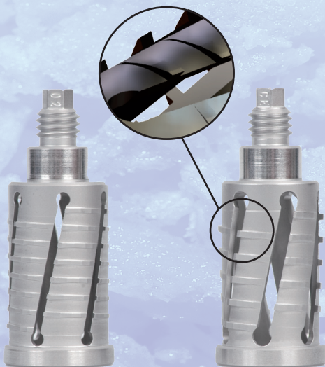
Two types of milling drums for various chip sizes. Each milling drum has spirally positioned teeth.
